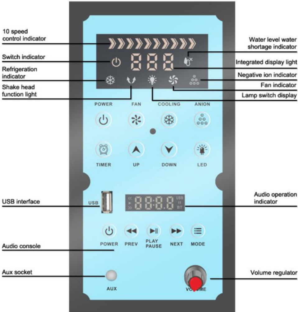
Gallery of Evaporative Cooler, AirMist16 with USB connector.
